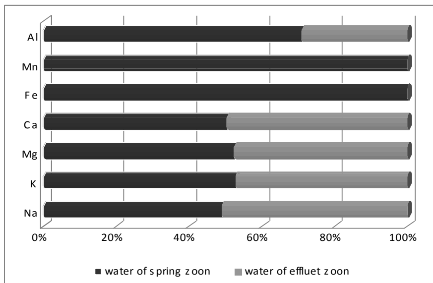
Fig. 4. The ratio of concentrations of macroelements in water in the spring zone to their concentrations in waters in the outflow zone
