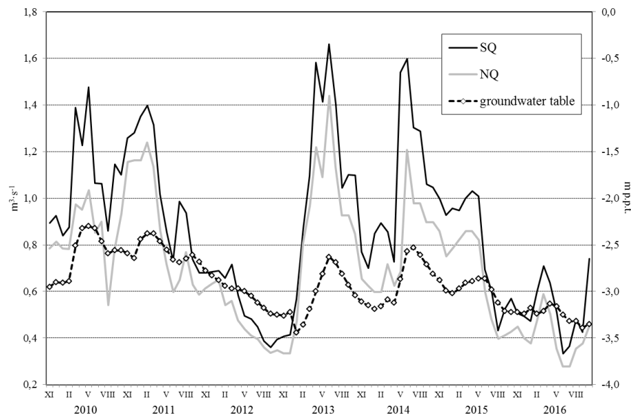
Fig. 5. Mean (SQ) and minimum (NQ) monthly discharge in the Krężniczanka River in Krężnica, and mean monthly groundwater table in Babin
