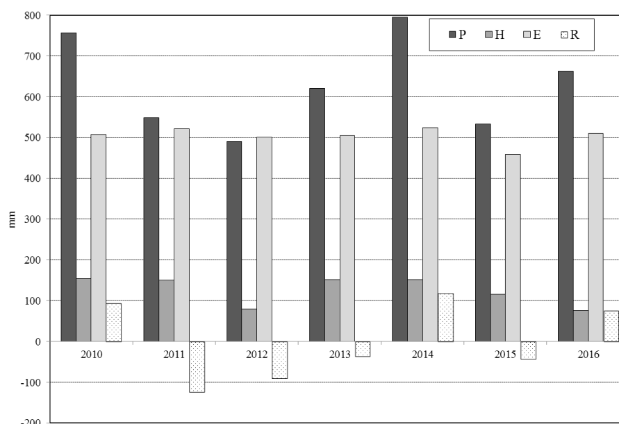
Fig. 7. Annual components of the water balance of the Krężniczanka River catchment: P – precipitation in Radawiec, H – runoff from the catchment to Krężnica, E – evapotranspiration, R – calculated state of retention
