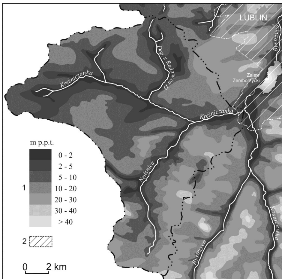
Fig. 3. Depth of occurrence of groundwater table: 1 – depth of occurrence of groundwater table, 2 – territory of Lublin
