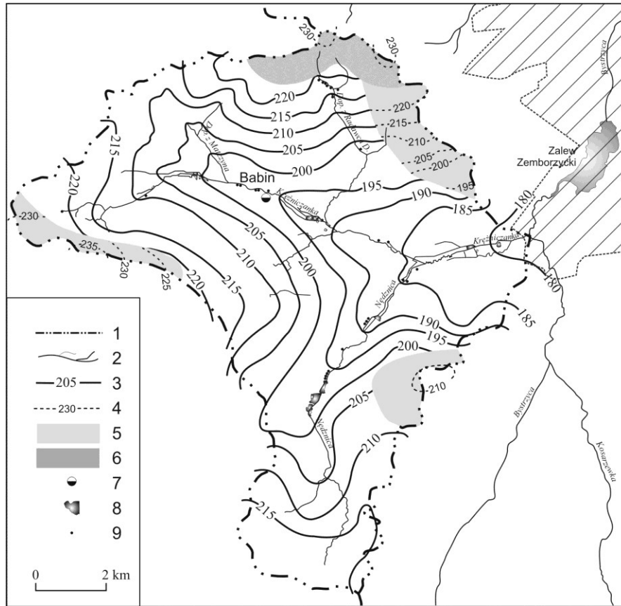
Fig. 4. Groundwater table levels: 1 – watershed, 2 – rivers, 3 – groundwater contour map of the main aquifer, 4 – groundwater contour map of the upper aquifer, 5 – area of occurrence of the upper aquifer in Cretaceous rocks, 6 – waters of the perched aquifer, 7 – groundwater monitoring station of the Polish Hydrogeological Survey, 8 – ponds and water bodies, 9 – springs
