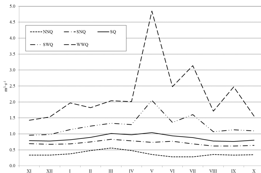
Fig. 6. Characteristic discharges of the Krężniczanka River in Krężnica in the years 2010–2016. Monthly discharge: NNQ – the lowest, SNQ – mean from the lowest values, SQ – mean, SWQ – mean from the highest values, WWQ – the highest
