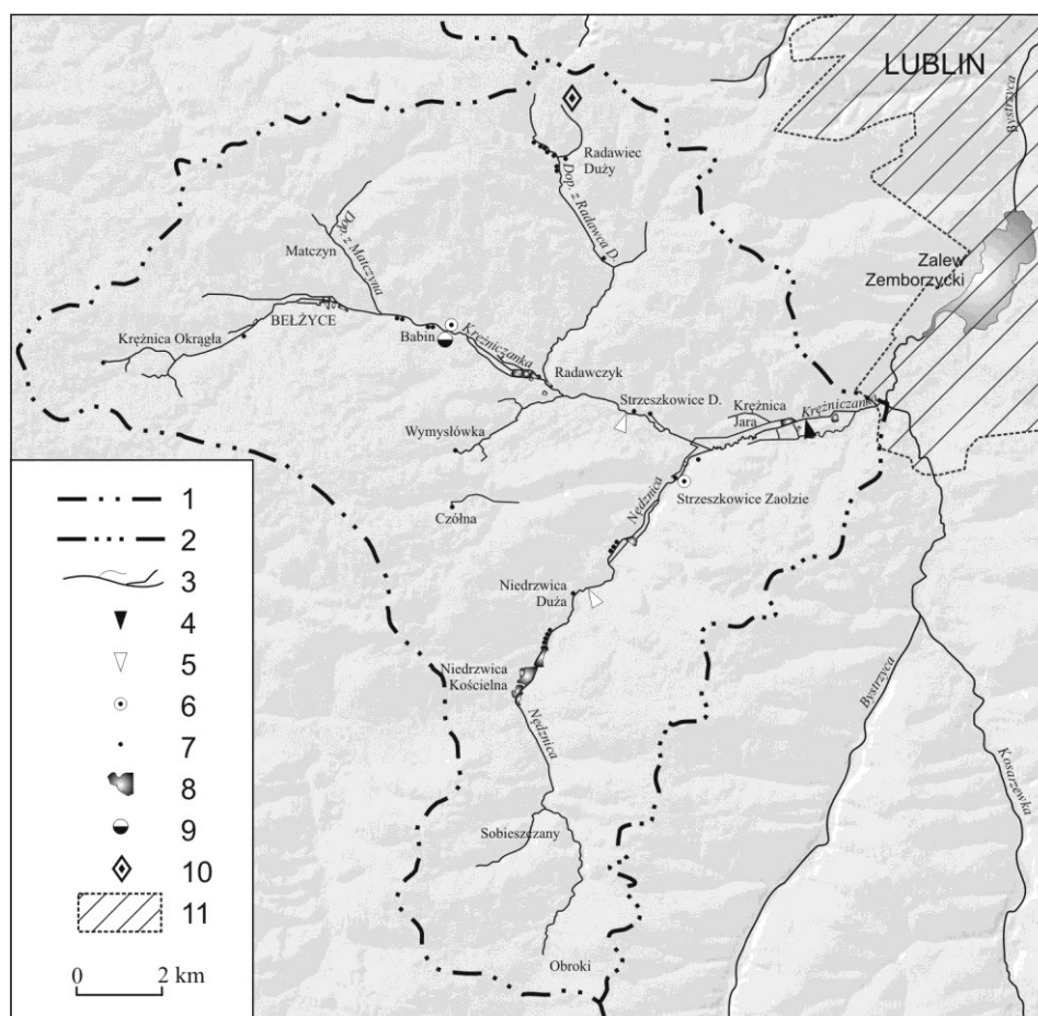
Fig. 2. River network and sites of hydrometric measurements in the Krężniczanka catchment: 1–2 – watersheds, 1 – II order, 2 – III order, 3 – rivers, 4 – water gauge, 5 – sites of periodical discharge measurements, 6 – springs with efficiency 10\text{--}30 \text{ dm}^3 \cdot \text{s}^{-1} , 7 – springs below 10 \text{ dm}^3 \cdot \text{s}^{-1} , 8 – ponds, 9 – groundwater monitoring station of the Polish Hydrogeological Survey, 10 – meteorological station of IMGW, 11 – territory of Lublin
