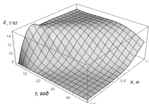
Fig. 7. Changes of air moisture content in the grain layer in time and according to a layer height
