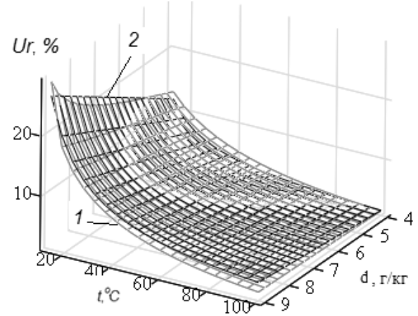
Fig. 1. Dependence of equilibrium grain moisture content on drying agent temperature and moisture content (1 – using the Henderson formula, 2 – using the formula (5))
