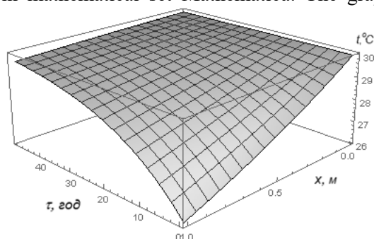
Fig. 4. Changes of air temperature in a grain layer in time and according to a layer height
