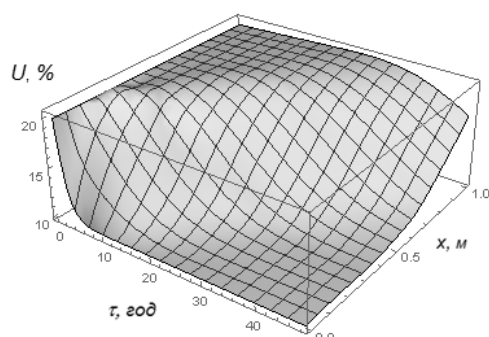
Fig. 5. Changes of grain moisture in time and according to a layer height
