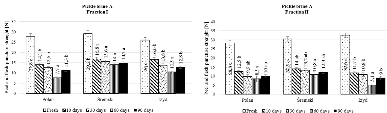
Fig. 2. Mean values of peel and flesh puncture strength in raw cucumbers and at the specific stages of pickling, relative to cucumber cultivar. Brine A.
