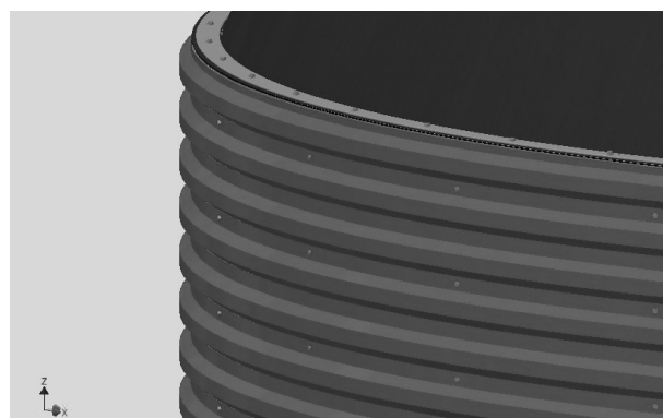
Fig. 18. Finished connection of trapezoidal sheet metal and sections [own elaboration]
