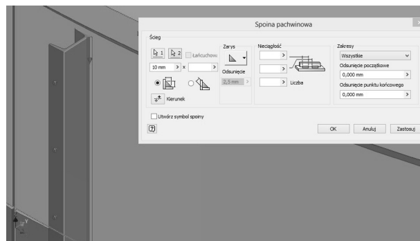
Fig. 20. Creation of continuous fillet weld connecting the tank's shell with the channel section [own elaboration]
