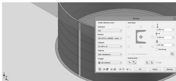
Fig. 14. Placement of the CH channel section 100x10 using section placement generator [own elaboration]
