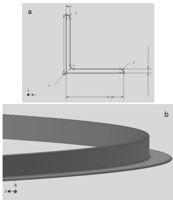
Fig. 4. Cross-section of the angle section 100x100x7; a – angle section sketch, b – rotation of the sketch by 360° [own elaboration]
