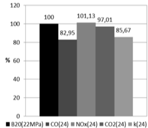
Fig. 3. Percentage presentation of the emission of toxic exhaust gas components for the engine fuelled with B20 biodiesel
