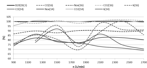
Fig. 5. Comparison of the percentages of toxic exhaust gas component emissions for an engine fuelled with B20 biodiesel at different values of fuel injection timing: 14, 16 and 18,5° of crankshaft revolutions before TDC (adopting the value of toxic exhaust gas component emissions at the ignition timing advance of 18.5° of crankshaft revolutions before TDC as a reference value, 100%), in the function of crankshaft rotational speed
