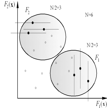
Fig. 4. Selection method VEGA [11, 14, 15]
